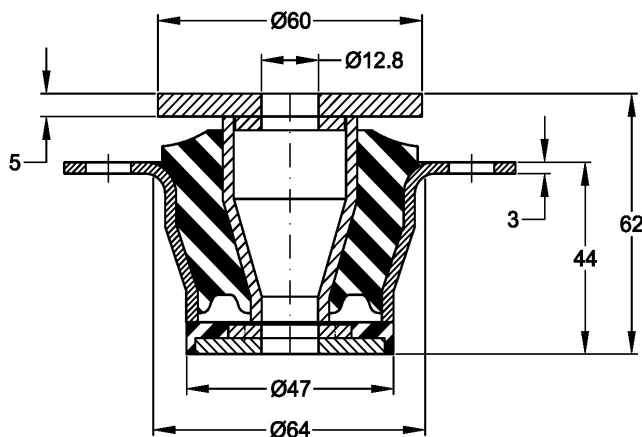
CROSS-SECTION
