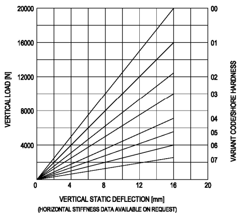
LOAD CHARACTERISTICS 10-TM-2000-H
