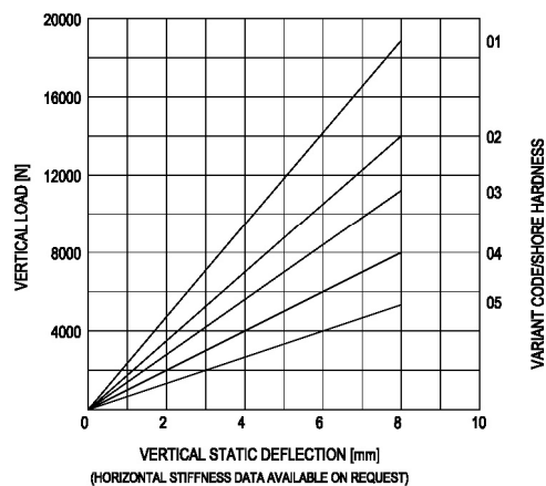
LOAD CHARACTERISTICS 10-TM-2000-N
